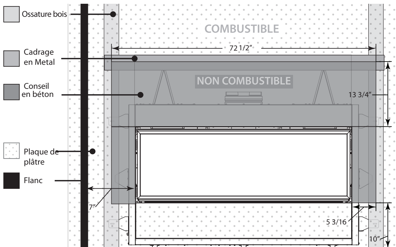
Figure 43: Zone Non-Combustible de finition
