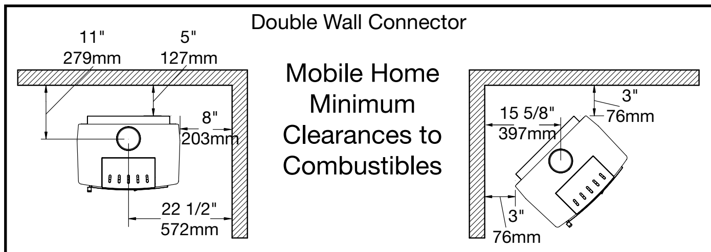
Figure 13: NEO2.5 mobile home clearances.
